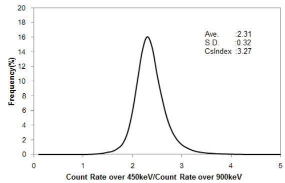
Fig. A3-23 Histogram of Cs-index in Shikoku
