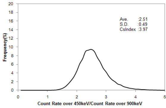
Fig. A3-28 Histogram of Cs-index in Chugoku 1
