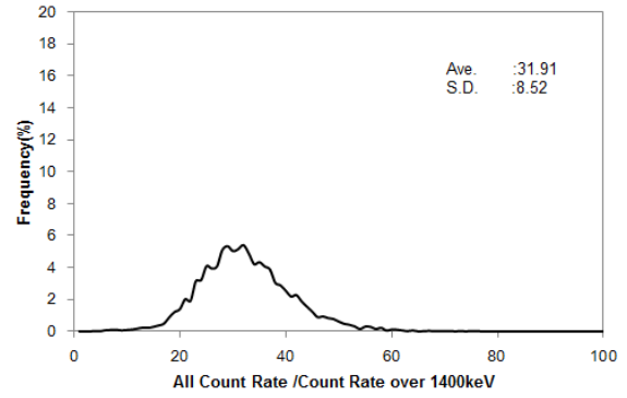
Fig. A3-2 Histogram of BG-index in Kyusyu 3
