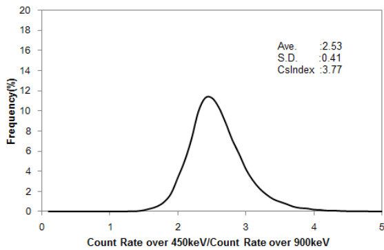
Fig. A3-26 Histogram of Cs-index in Kinki 3
