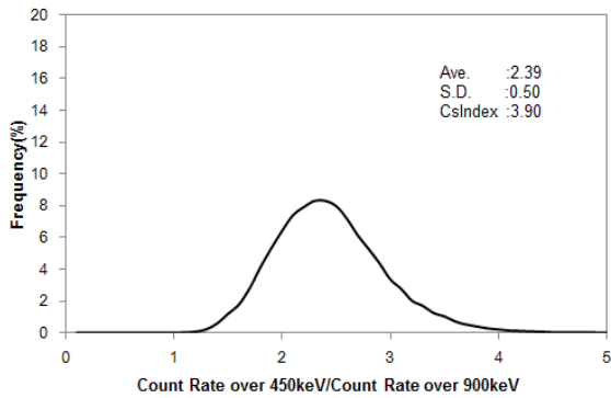
Fig. A3-32 Histogram of Cs-index in Hokkaido 2
