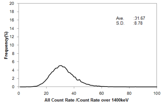
Fig. A3-8 Histogram of BG-index in Chugoku 1
