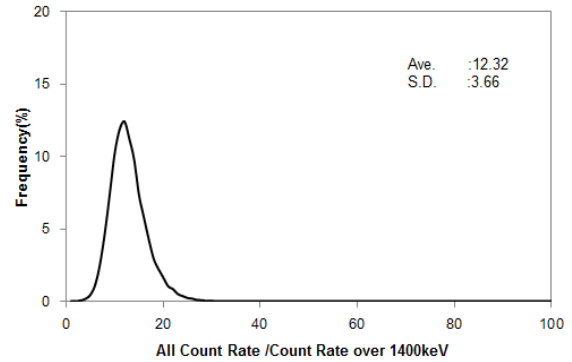
Fig. A3-12 Histogram of BG-index in Hokkaido 3
