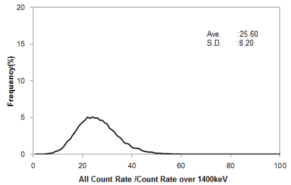
Fig. A3-10 Histogram of BG-index in Hokkaido 2
