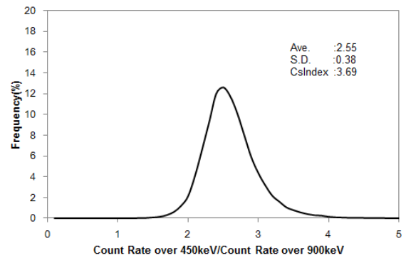
Fig. A3-27 Histogram of Cs-index in Kinki 4
