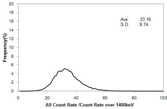
Fig. A3-3 Histogram of BG-index in Kinki 1
