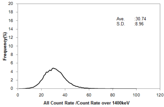
Fig. A3-7 Histogram of BG-index in Kyusyu 1
