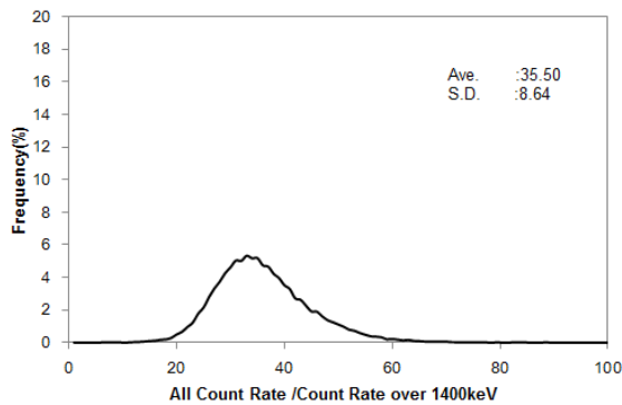
Fig. A3-5 Histogram of BG-index in Kinki 4
