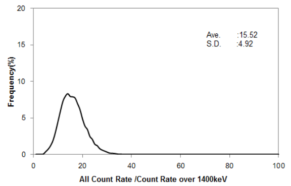
Fig. A3-14 Histogram of BG-index in Hokkaido 4
