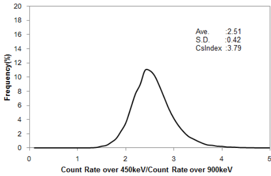
Fig. A3-24 Histogram of Cs-index in Kinki 1
