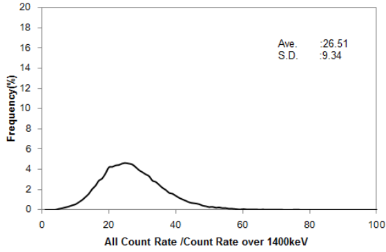
Fig. A3-1 Histogram of BG-index in Kyusyu 2
