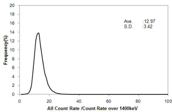
Fig. A3-15 Histogram of BG-index in Chugoku 2
