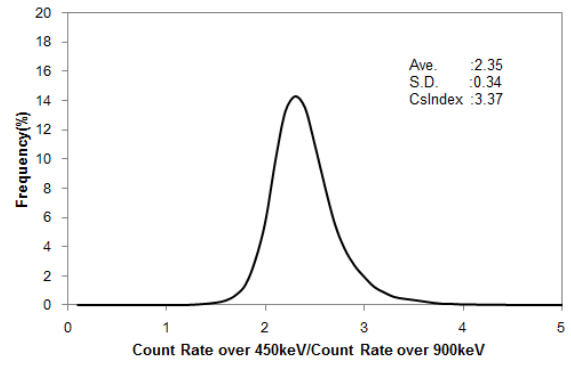
Fig. A3-29 Histogram of Cs-index in Chugoku 2
