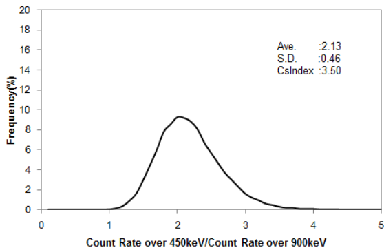
Fig. A3-34 Histogram of Cs-index in Hokkaido 4
