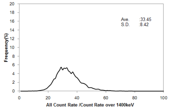
Fig. A3-4 Histogram of BG-index in Kinki 3
