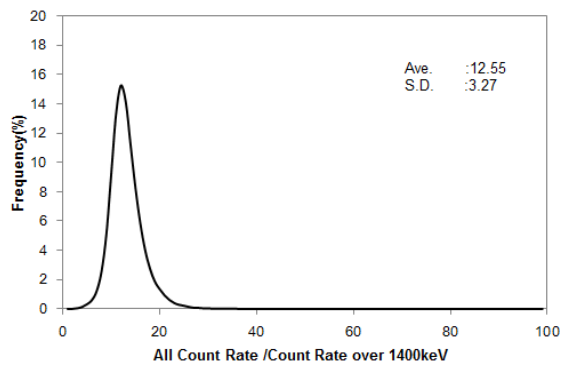
Fig. A3-13 Histogram of BG-index in Shikoku 1
