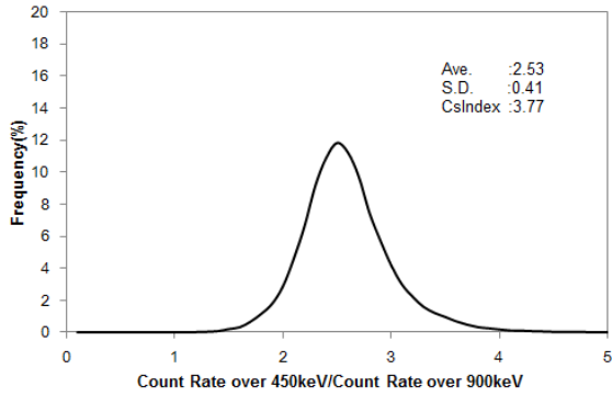
Fig. A3-30 Histogram of Cs-index in Chugoku 3
