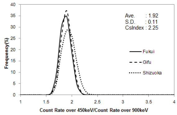
Fig. A3-19 FUGURO; Histogram of Cs-index
