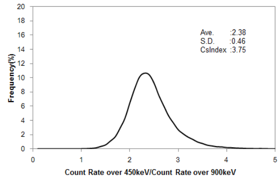
Fig. A3-33 Histogram of Cs-index in Hokkaido 3
