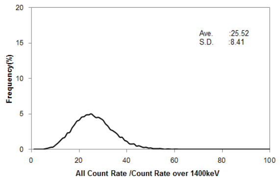
Fig. A3-6 Histogram of BG-index in Hokkaido 1
