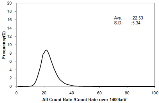
Fig. A3-11 Histogram of BG-index in Kinki 2
