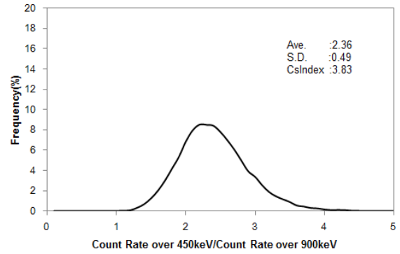
Fig. A3-31 Histogram of Cs-index in Hokkaido 1
