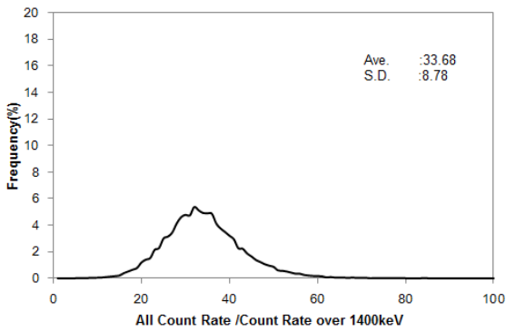
Fig. A3-9 Histogram of BG-index in Chugoku 3
